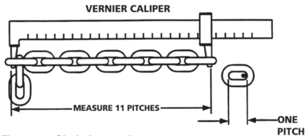
Figure 5 - Chain Inspection
